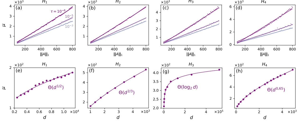
Figure E1: Scaling of \mu , the number of matrix-vector multiplications. (a)-(d) The scaling of \mu with \|A\|_1 for Hamiltonians H_j , j = 1, 2, 3, 4 , when considering several error tolerances \tau . (e)-(h) The scaling of \mu with dimension d when considering \tau = 10^{-8} for each H_j , respectively. In all figures, dots are sampling data and solid lines are fitting curves. The parameters setup of H_1 , H_2 are the same as the ones given in the captions of Figs. 2, 3. Parameters of H_3 and H_4 are as follows: for H_3 , E_{Ci}/2\pi = 2.5 GHz, E_{Ji}/2\pi = 8.9 GHz, E_{Li}/2\pi = 0.5 GHz, g/2\pi = 0.1 GHz and \phi = 0.33 ; for H_4 , a_x^{(\nu)}/2\pi = a_y^{(\nu)}/2\pi = 0.5 GHz and g/2\pi = 0.1 GHz.
