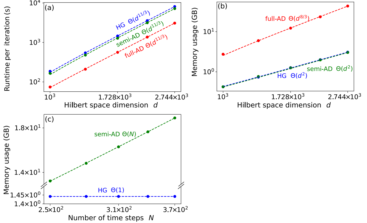
Figure 3: Benchmark results for unitary gate optimization in a system consisting of three coupled transmons. (a) Runtime per iteration and (b) memory usage versus Hilbert space dimension d . The total Hilbert space dimension d is increased by enlarging the cutoff of each transmon from 10 to 14 simultaneously. (c) Memory usage as a function of the number of time steps for d = 12^3 = 1728 . Full-AD (not shown) would require more memory than our resources (estimated: 1TB). All plots are in log-log scale. Dashed lines are power-law fits. (Parameters: g/2\pi = 0.1 GHz, \alpha/2\pi = -0.225 GHz and a^{(\nu)}/2\pi = 0.1 GHz.)
