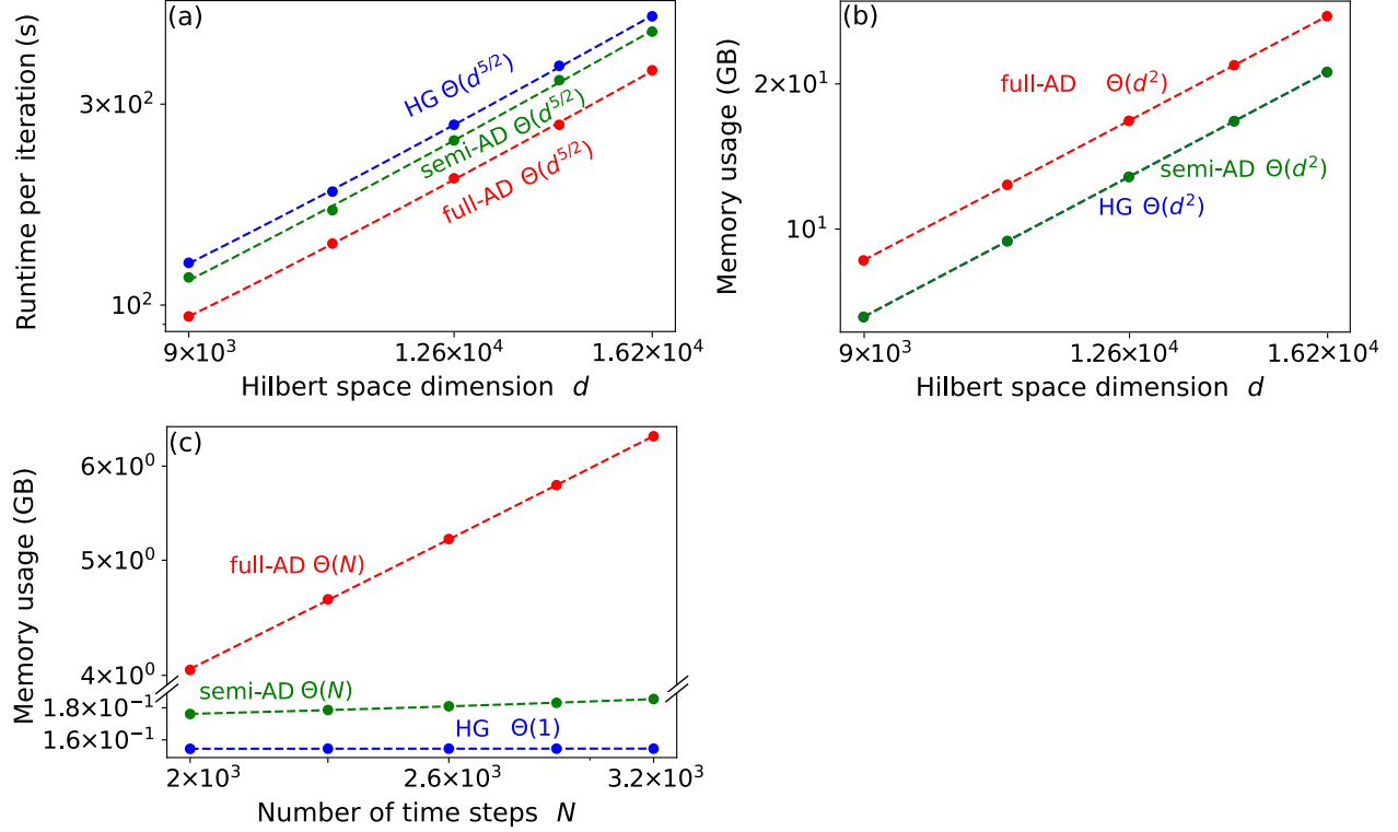
Figure 2: Benchmark results for Fock state generation in a system consisting of a cavity coupled to a transmon. (a) Runtime per iteration and (b) memory usage versus Hilbert space dimension d . The dimension is varied by increasing cavity dimension while fixing the transmon dimension to 6. (c) Memory usage as a function of the number of time steps for d = 240 . All plots are in log-log scale. Dashed lines are power-law fits. (Parameters: \Delta/2\pi = 3 GHz, g/2\pi = 0.1 GHz, \alpha/2\pi = -0.225 GHz and constant controls a_z/2\pi = a_x/2\pi = 0.1 GHz.)
