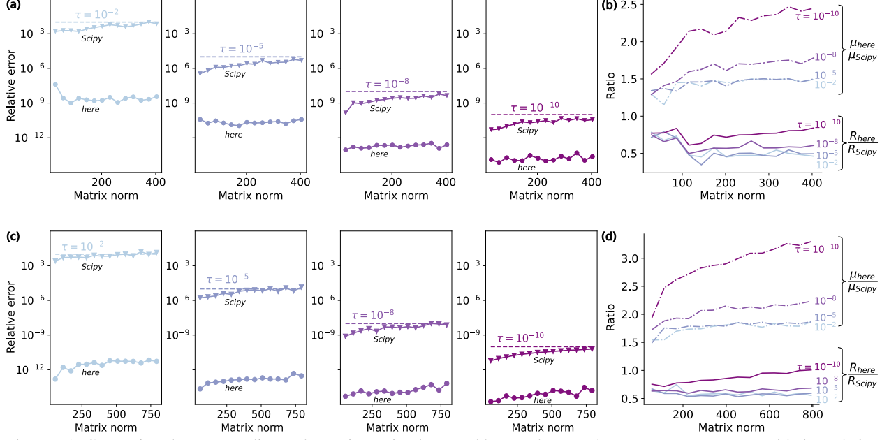
Figure D1: Comparison between scaling and squaring as implemented here and SciPy’s expm_multiply , considering relative error and runtime. (a), (c) Relative error versus matrix norm. (b), (d) Ratios of runtime and \mu (i.e. number of matrix-vector multiplications) between our and SciPy’s implementations as functions of the matrix norm. The matrix norm \| -iH\Delta t \|_2 is varied by increasing \Delta t \in [1, 10] . In all panels, colors encode different error tolerances \tau . The results of the first and second row are obtained based on cavity-transmon and three coupled transmons Hamiltonians, respectively. The system parameters of these two Hamiltonian are the same as the ones given in the captions of Figs. 2, 3, respectively.
